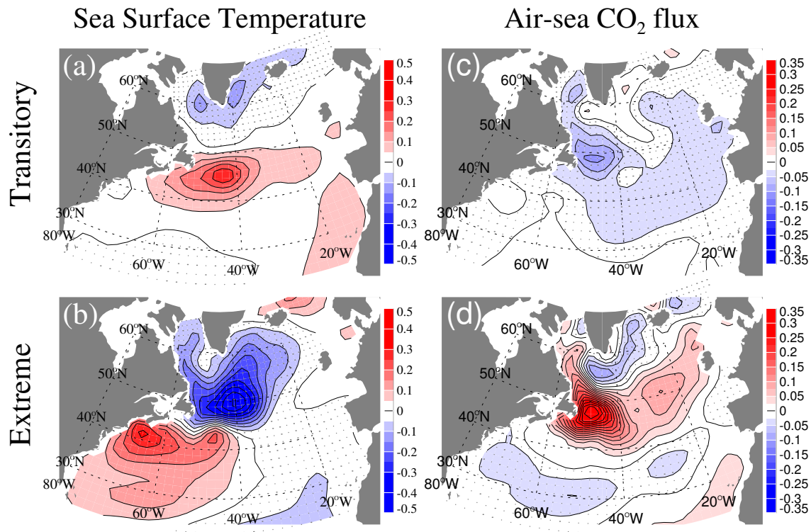
Fig. 9. Anomalies of SST [°C] for the decadal mode during the (a) transitory and (b) extreme phases of the 8-phase cycles. Corresponding maps are also shown for the (c) transitory and (d) extreme phases for anomalies of the air-sea CO 2 flux [mol C m -2 year -1 ]. Negative values are indicated by dotted areas. A transitory phase occurs a quarter of a cycle before an extreme phase.
