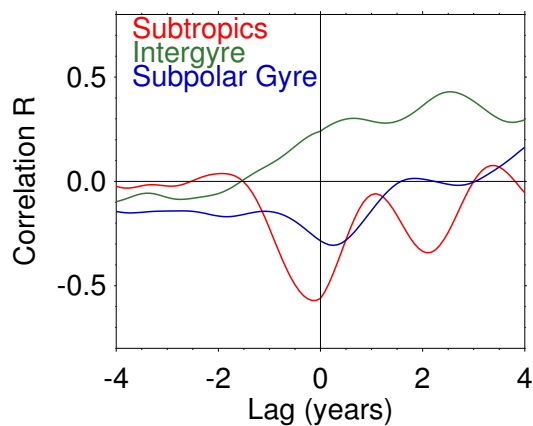
Fig. 5. Lag correlation between the NAO index and the air-sea CO 2 flux in the subtropical region, bounded by 65° W–43° W and 29° N–37° N (red) as well as the intergyre region, bounded by 54° W–21° W and 45° N–52° N (green), and the subpolar region bounded by (65° W–43° W, 55° N–60° N) (blue). White noise was removed by MSSA prior to this lag correlation analysis (see Sect. 2.3).
