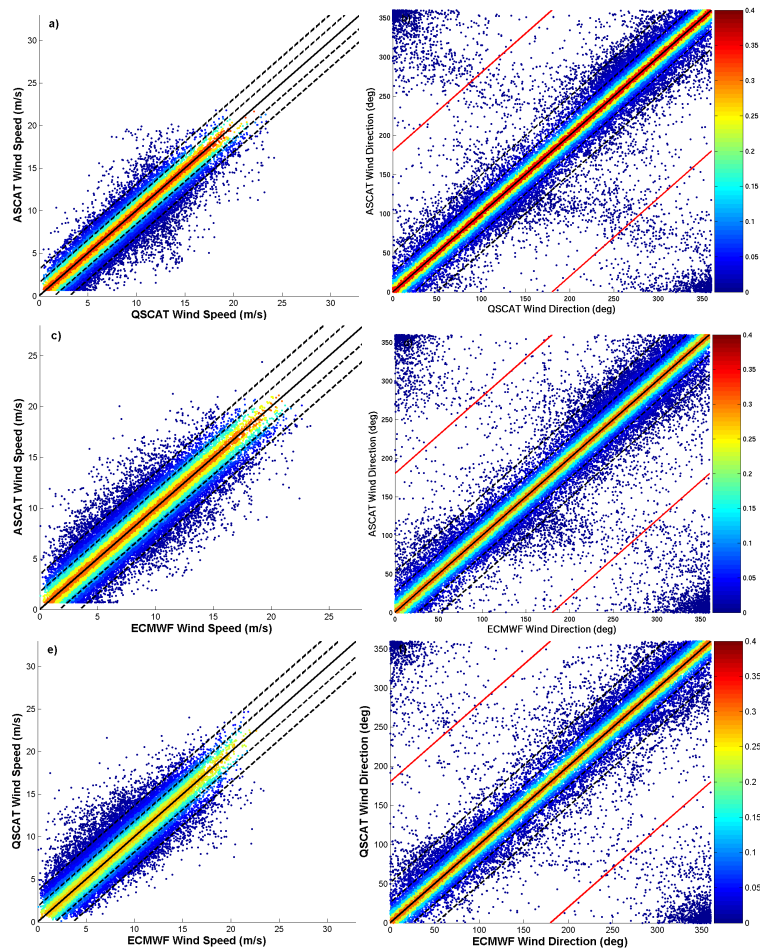
Fig. 3. Scatterplots of wind speeds (left column) and directions (right column) derived from QuikSCAT and ASCAT (top), ECMWF and ASCAT (middle), and from ECMWF and QuikSCAT (bottom).
