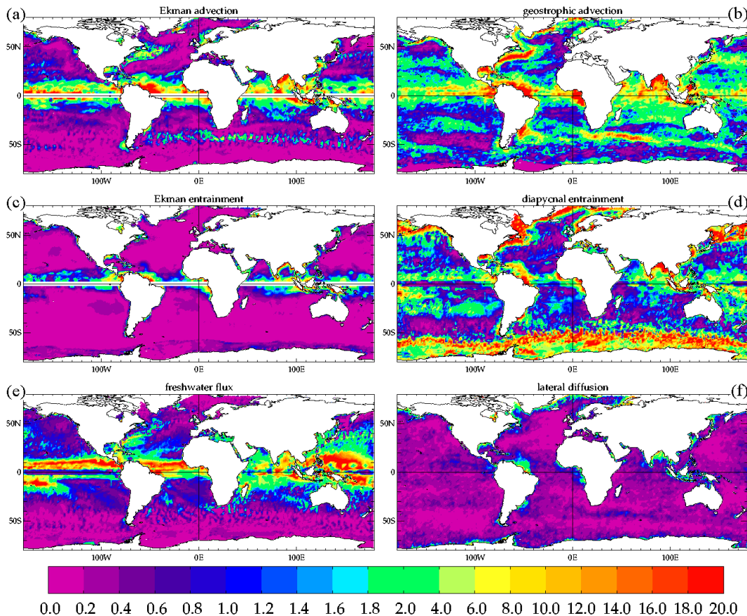
Fig. 10. Annual RMS of the daily values of the salinity balance terms (in 10^{-3} psu.day ^{-1} ) from the simulation. (a) Ekman advection, (b) geostrophic advection, (c) Ekman entrainment, (d) diapycnal entrainment, (e) surface freshwater flux, (f) lateral diffusion. The color scale is nonlinear, with intervals of 0.2 for 0 < \partial_t S < 2 and 2.0 for 2 < \partial_t S < 20 .
