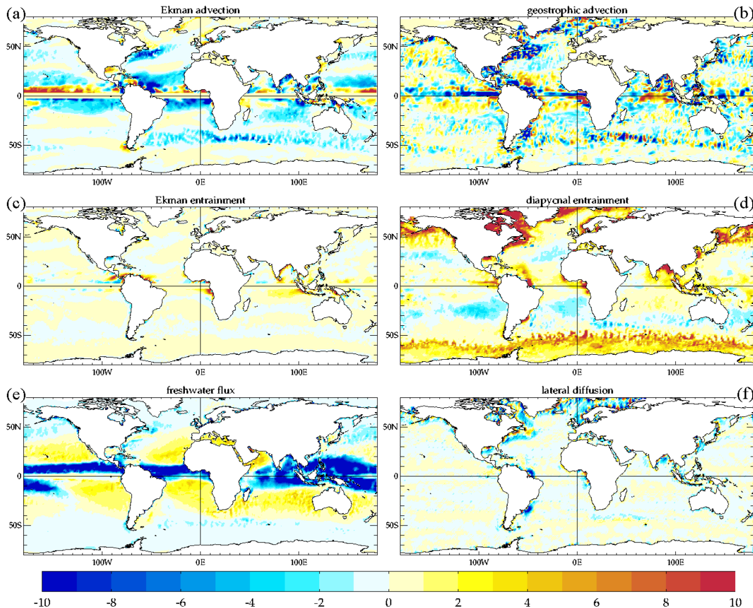
Fig. 9. Annual mean of the salinity balance terms (in 10^{-3} psu.day ^{-1} ) from the simulation. (a) Ekman advection, (b) geostrophic advection, (c) Ekman entrainment, (d) diapycnal entrainment, (e) surface freshwater flux, (f) lateral diffusion. The colour scale is linear, with blue levels indicating an annual freshening ( \partial_t S < 0 ) and red levels indicating an annual salinisation ( \partial_t S > 0 ).
