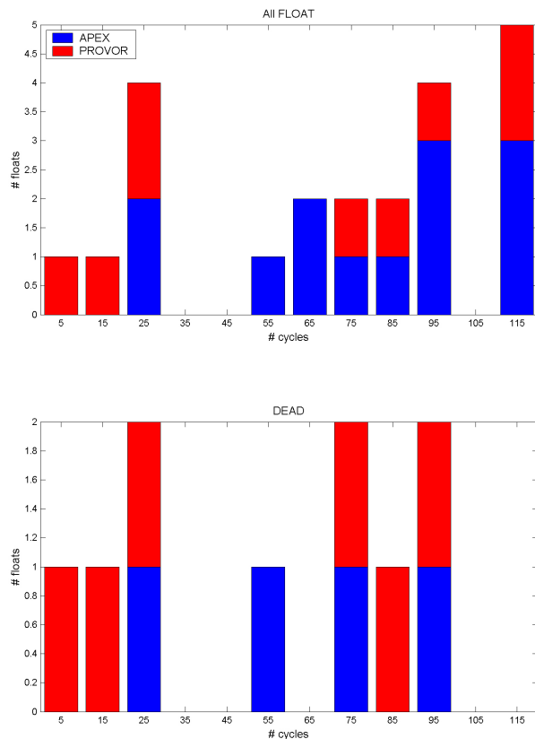
Fig. 3. Histograms of the number of cycles carried out by all the MEDARGO profilers between July 2004 and March 2006 (a) . Same histogram for the profilers that stopped transmitting before 31 March 2006 (b) .
