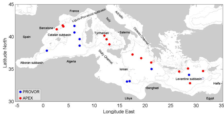
Fig. 2. Deployment locations of the MEDARGO profilers released between July 2004 and March 2006 throughout the Mediterranean Sea. The 1000 and 2000-m isobaths are shown with grey curves.
