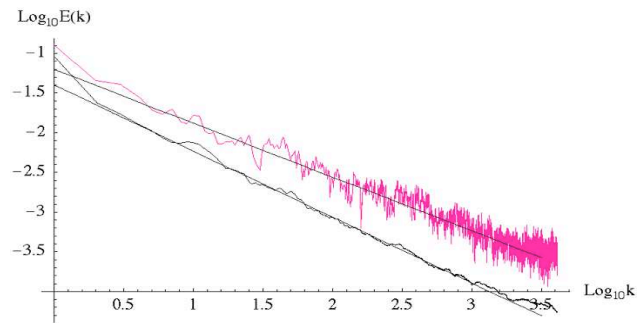
Fig. 24d. Comparisons of ensemble spectra for 16 realizations of the Turcotte (black) model and 16 realizations of the binomial/ p model (pink) with \mu\epsilon_+=1.5 along with theoretical slopes ( 0.83=2(1-\log_2 \mu\epsilon) , 0.678=1-K(2)=1-\log_2 \langle \mu\epsilon^2 \rangle , respectively).
