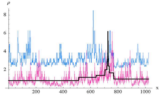
Fig. 24c. Turcotte model (black), binomial/ p model (pink), \alpha model (blue) (offset by 2 units for clarity). All models have the same parameters: the de Wijs values: d=0.2 hence \mu\epsilon_+=1.2 (hence \gamma_+=0.27 for alpha model).
