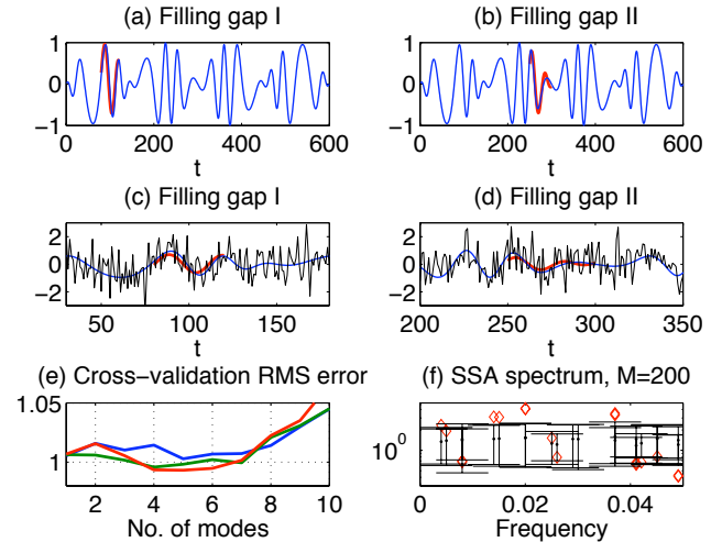
Fig. 2. Gap filling of (a, b) a nonlinear oscillatory signal s(t) , and (c, d) of its noise-contaminated version x(t) (black line); see Eq. (6), units are nondimensional. Blue line is the oscillatory component s(t) , red is the filled-in data. Gap I is over the interval 80 \leq t \leq 120 , while gap II is over 250 \leq t \leq 300 . (e) Cross-validation results for filling gap II in x(t) ; blue, green and red lines are for SSA windows of M=160 , 180 and 200, respectively. (f) Monte-Carlo SSA spectra of x(t) with window M=200 (see caption to Fig. 1).
