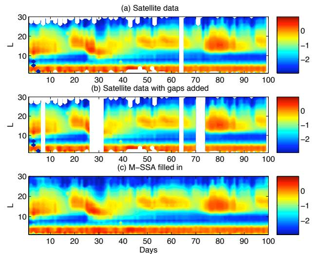
Fig. 5. CRRES satellite measurements of 1MeV high-energy electron fluxes ( \text{sr} \cdot \text{MeV} \cdot \text{s} \cdot \text{cm}^2 ) ^{-1} in Earth’s radiation belts as a function of L-shell: (a) original data with missing values in white; (b) original data with a few synthetic gaps added; and (c) M-SSA filled-in. The L-shell parameter measures distance to the intersection between a magnetic-dipole field line and the equatorial plane in Earth radii; it indicates how far trapped electrons are from the Earth.
