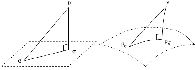
Fig. 4. The left figure depicts the optimization procedure in the Gaussian framework. The first guess (actually the null vector \mathbf{0} ) is projected orthogonally onto the space of sources which satisfy the measurement constraints. The true source \sigma belongs to this space. The right figure depicts the optimization for a general prior within the maximum entropy on the mean approach. The prior \nu is “projected” onto the manifold of the exponential laws, the average of which satisfies the measurement constraints. The exponential law whose first moment is the true source belongs to this manifold.
