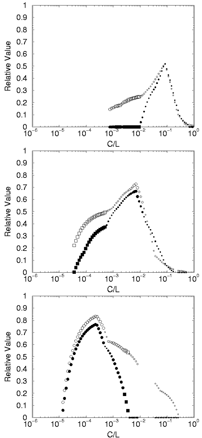
Fig. 15. Same as Fig. 11, but for morning precipitation (+84 h to +96 h).
