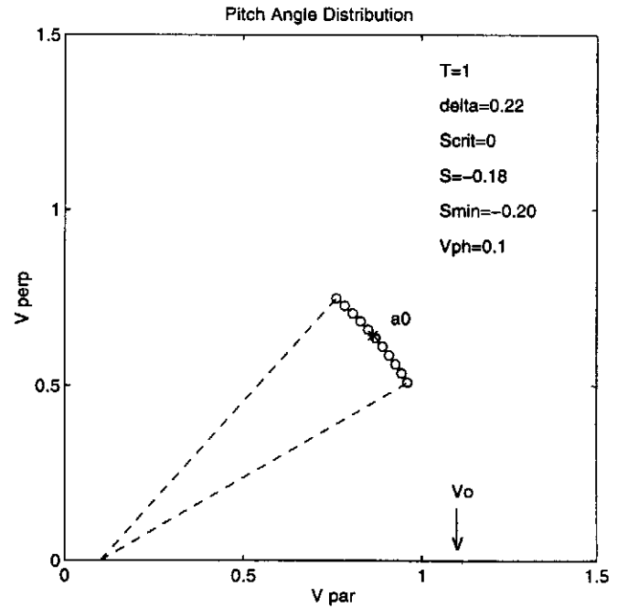
Fig. 5. Theoretical particle distribution in the (V_{\parallel}, V_{\perp}) plane displaying the pitch-angle width for a constant value of the second invariant of the movement S(\alpha, \psi) . V_0 is the initial velocity of the cyclotron resonant beam ( T=1 ).
