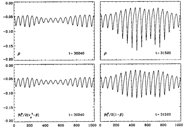
Fig. 15. Snapshots of the density \rho (corrected by a constant) from the primitive MHD equations (top) and the corresponding adiabatic prediction (bottom), for \beta = 1.5 , amplitude \epsilon^{1/2} = 0.25 , k = \epsilon = 0.0625 and right-hand polarization.
