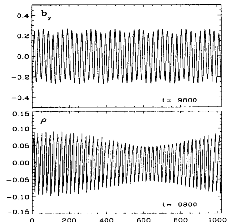
Fig. 16. Snapshots of the magnetic field b_y (top) and of the density \rho (bottom) obtained from the primitive MHD equations, for \beta = 0.5 , amplitude \epsilon^{1/2} = 0.25 , k = \epsilon = 0.0625 and left-hand polarization.
