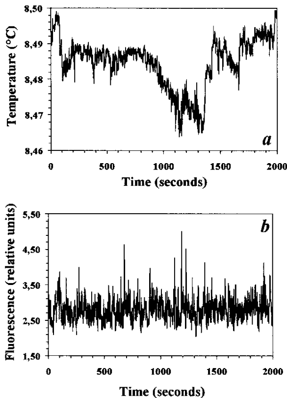
Fig. 1. A portion of temperature (a) and in vivo fluorescence (b) time series recorded in the Southern Bight of the North Sea. Sharp fluctuations occurring on all time scales are clearly visible, indicating the intermittent behaviour of the dataset.
