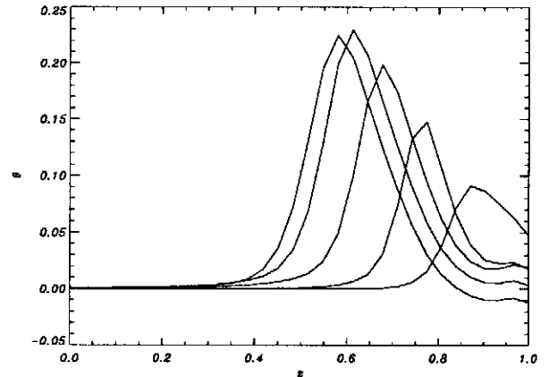
Fig. 2. Vertical profile of temperature fluctuation inside a jet (Run III), at x=0 .
