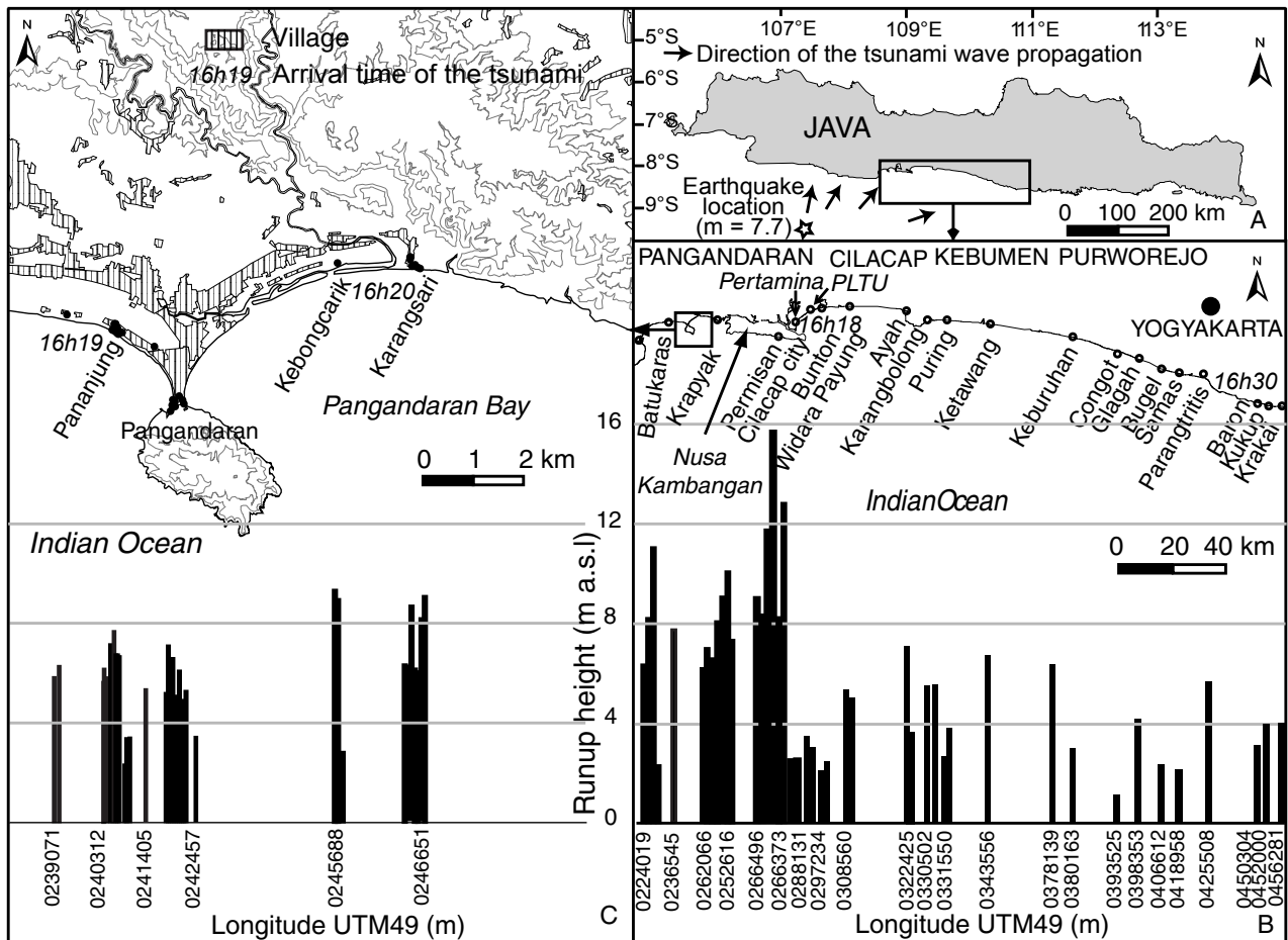
Fig. 1. Runup heights distribution of the 17 July 2006 tsunami along the south coast of Java. (A) Location of the field study in Java with indication of the 17 July 2004 earthquake epicentre. (B) Runup heights distribution and arrival time at selected spots along the Javanese coastline. (C) Zoom at the Pangandaran district.
