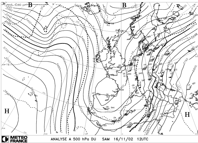
Fig. 5. 16 November 2002 12:00 UTC, analysis at 500 hPa: geopotential (in m) and temperature (in °C) are drawn, respectively, as solid and dashed lines (H for high centre and B for low centre of geopotential).
