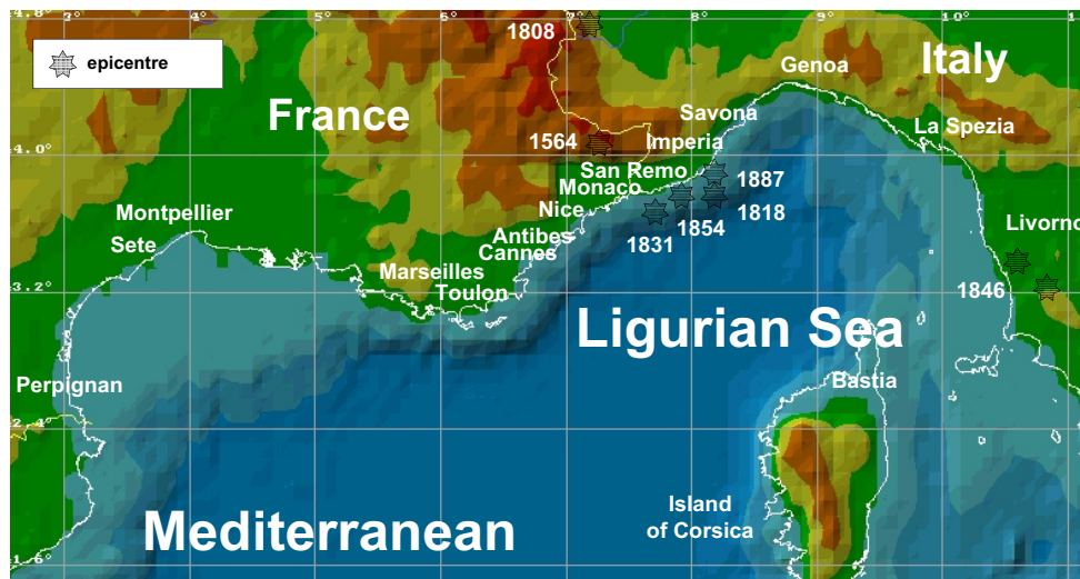
Fig. 1. Epicentres of earthquakes induced tsunami on the French coast of Mediterranean.
