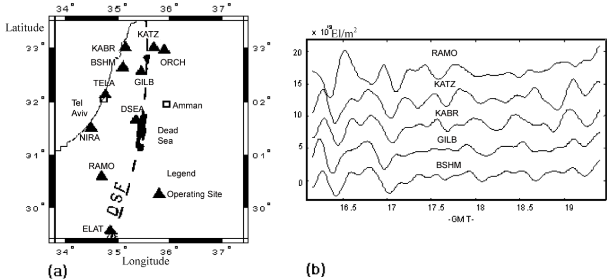
Fig. 4. (a) Map of the GIL network (b) Decomposition of TEC observations obtained from one satellite at five GIL receivers. The similarity of the signal at the KATZ, KABR, GILB and BSHM sites, which are located between 30–60 km apart, is obvious. In contrast, the RAMO site is located 240 km from these and shows a different signal.
