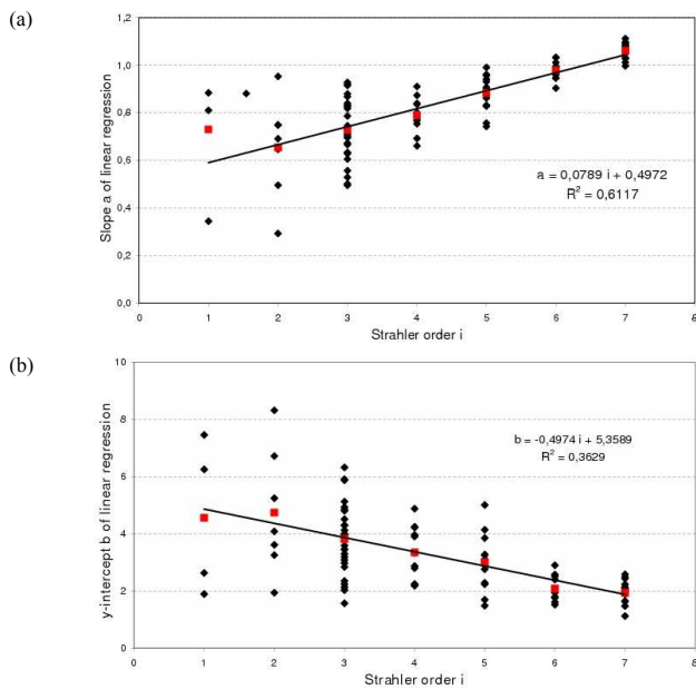
Fig. 5. Relationship to Strahler order of the slope a and y-intercept b of the linear regression between WT and lagged AT , using the lag that maximizes the determination coefficient R^2 . The black lines are the regression lines between the Strahler orders and the means of the slope and y-intercept for each Strahler order, represented by red squares. They are characterized by the linear regression equations and determination coefficients given in the plots.
