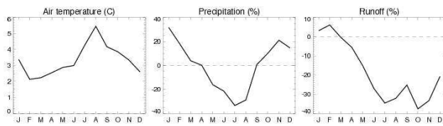
Fig. 3. Monthly mean anomalies between the climate change and reference scenarios (A2-REF), on average over the entire Seine watershed, for temperature (in °C), precipitation and runoff simulated by the CLSM (relative anomalies in % of the monthly mean reference value).
