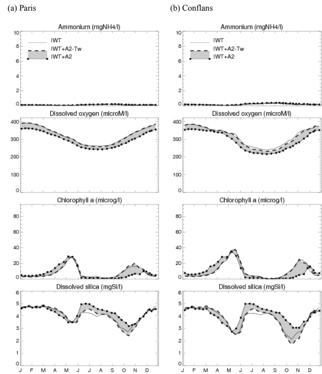
Fig. 9. Impact of climate change simulated by RIVERSTRAHLER on water quality in Paris and Conflans (interannual monthly means over 5 years), with reduced point source input as anticipated for 2050. Chlorophyll- a is proportional to phytoplankton biomass (Garnier et al., 1995). The differences between simulations IWT and IWT+A2-Tw show the impact that arises from the changes in river discharge, and the differences between IWT+A2-Tw and IWT+A2, shaded in grey, show the impacts that are driven by the warming of the water column.
