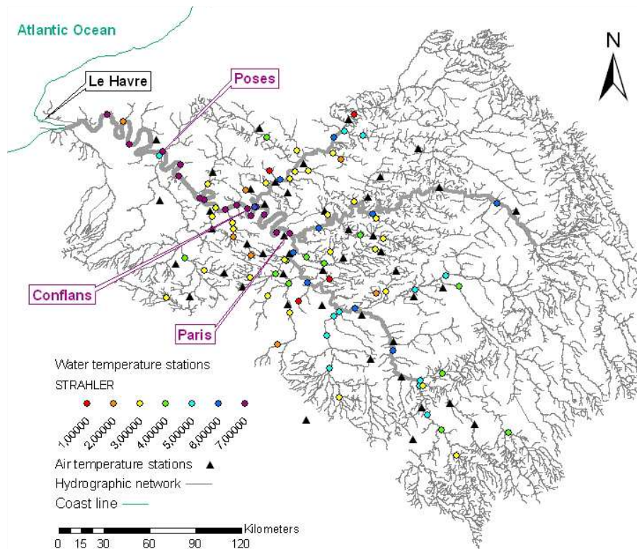
Fig. 1. Map of the Seine River basin, locating the monitoring stations of air and water temperature. The colours of the latter indicate the Strahler order at the water temperature measurement stations. The hydrographic network appears in grey and is thicker at Strahler orders 6 and 7. The Seine has an order 7 at Conflans, as in Paris, but the corresponding dot is masked by the one of the most downstream station on the Oise tributary, of order 6.
