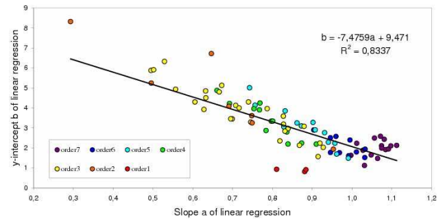
Fig. 6. Relationship between the slope a and y-intercept b of the linear regression between WT and lagged AT , using the lag that maximizes the determination coefficient R^2 . The color of the dots indicates the Strahler order at the WT measurement stations. The black line is the regression line between the slopes and y-intercepts, characterized by the displayed linear regression equation and determination coefficient.
