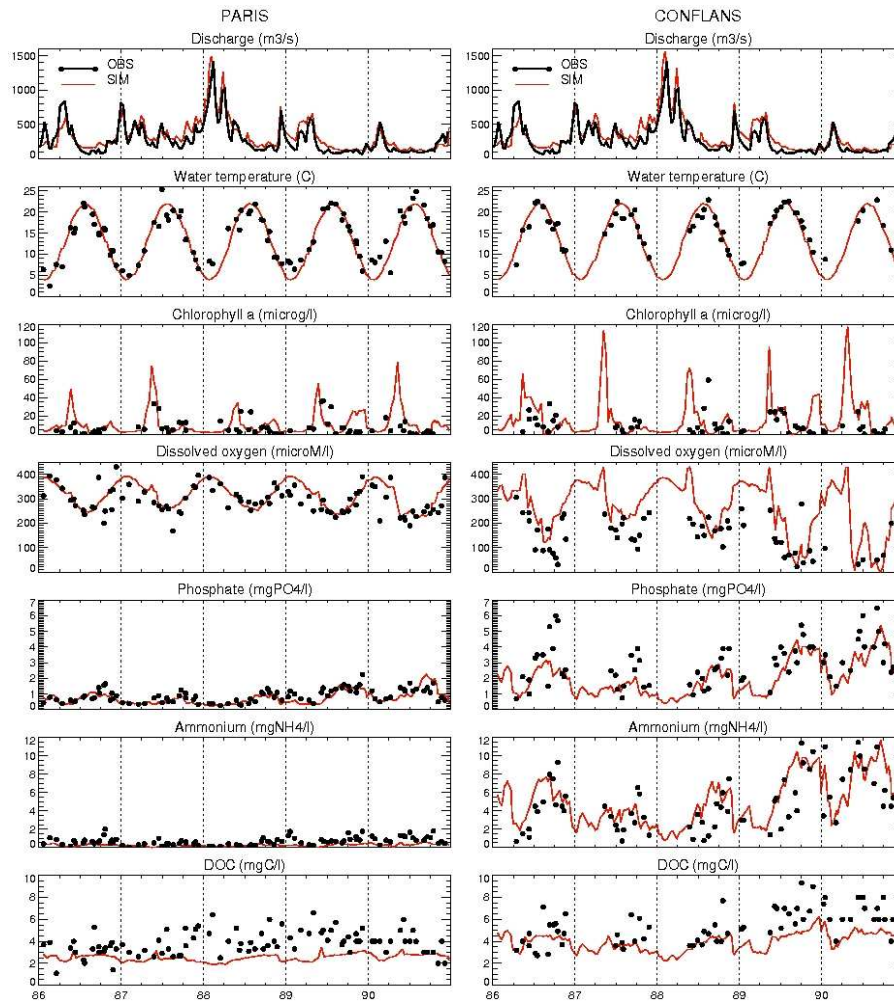
Fig. 2. Validation of the discharge and biogeochemical water quality simulated by RIVERSTRAHLER coupled to CLSM in 1986–1990, in Paris and Conflans: comparison of observations (black dots; source: Réseau National de Bassins) with the water quality simulated using point sources of year 1991. Chlorophyll a is proportional to phytoplankton biomass (Garnier et al., 1995). DOC stands for dissolved organic carbon. Discharge is not measured at Conflans, and the observed values at Paris are used instead, as the upstream contributing areas to the two stations are almost identical.
