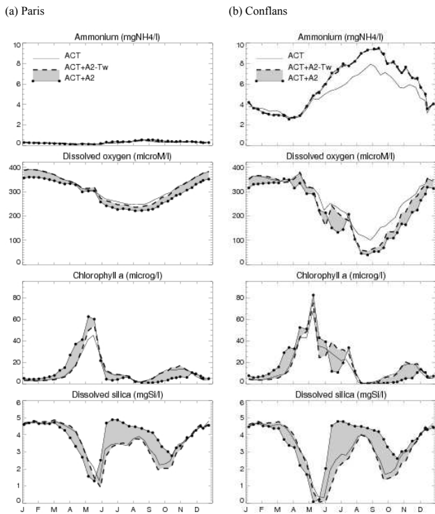
Fig. 8. Impact of climate change simulated by RIVERSTRAHLER on water quality in Paris and Conflans (interannual monthly means over 5 years), with point source input from 1991. Chlorophyll- a is proportional to phytoplankton biomass (Garnier et al., 1995). The differences between simulations ACT and ACT+A2-Tw show the impact that arises from the changes in river discharge, and the differences between ACT+A2-Tw and ACT+A2, shaded in grey, show the impacts that are driven by the warming of the water column.
