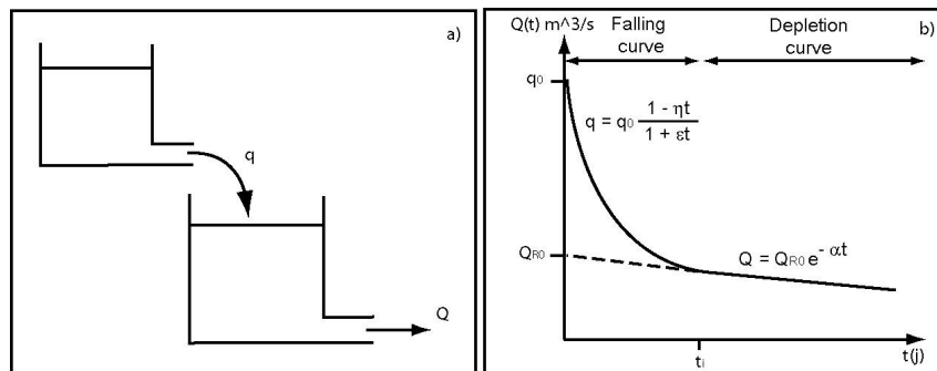
Fig. 4. (a) two reservoirs model and (b) decomposition of recession proposed by Mangin (1970).
