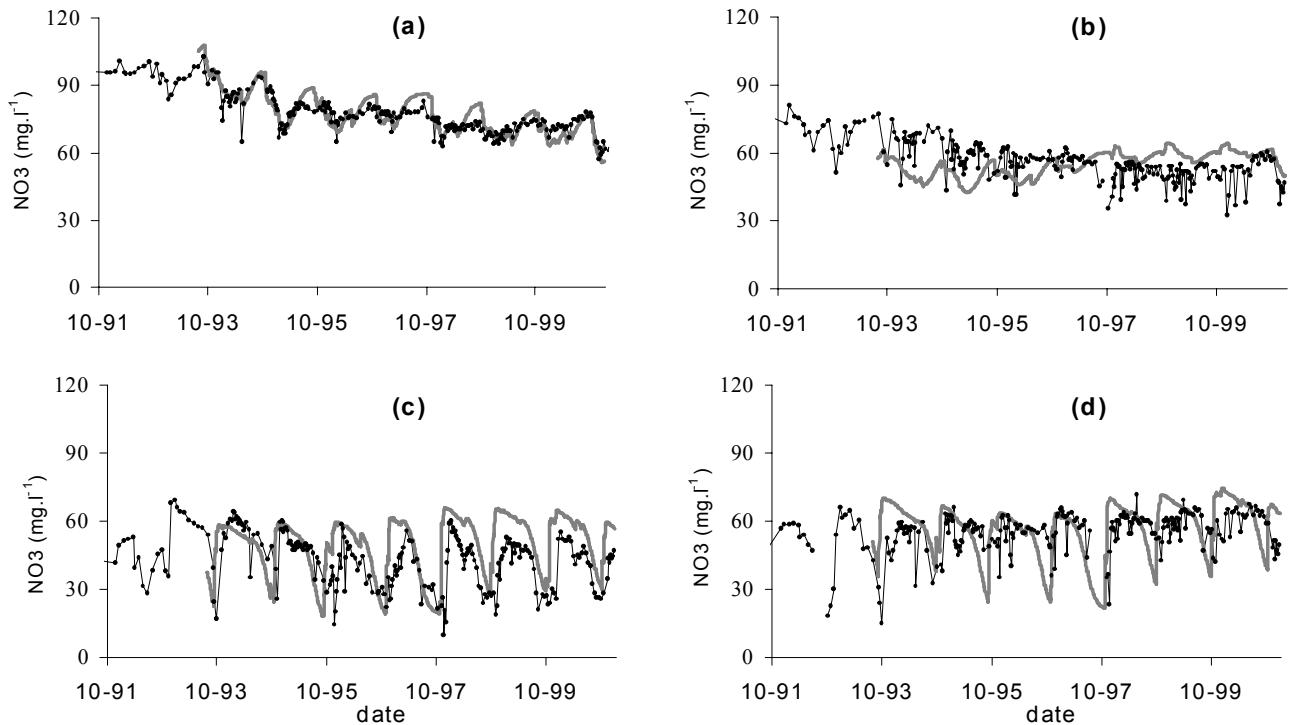
Fig. 4. Simulated (grey line) and observed (black points) concentrations ( \text{mg}\cdot\text{l}^{-1} ) for the Kerbernez (a), Le Puits (b), Coat Timon (c) and Kerrien (d) catchments
