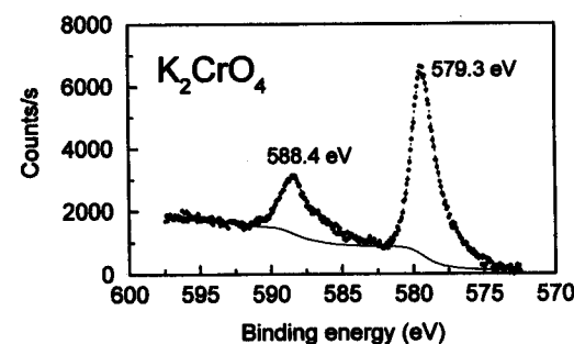
Fig. 2. XPS analyses of the end products compared with those of Cr 2 O 3 and K 2 CrO 4 : Cr 2p spectra. (a) obtained from Fe(OH) 2 and (b) obtained from GR(SO 4 2- ).
