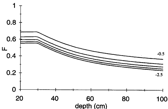
Fig. 7. Influence of the critical leaf potential on F . The five curves correspond to -0.5, -1.0, -1.5, -2.0, -2.5 MPa.
