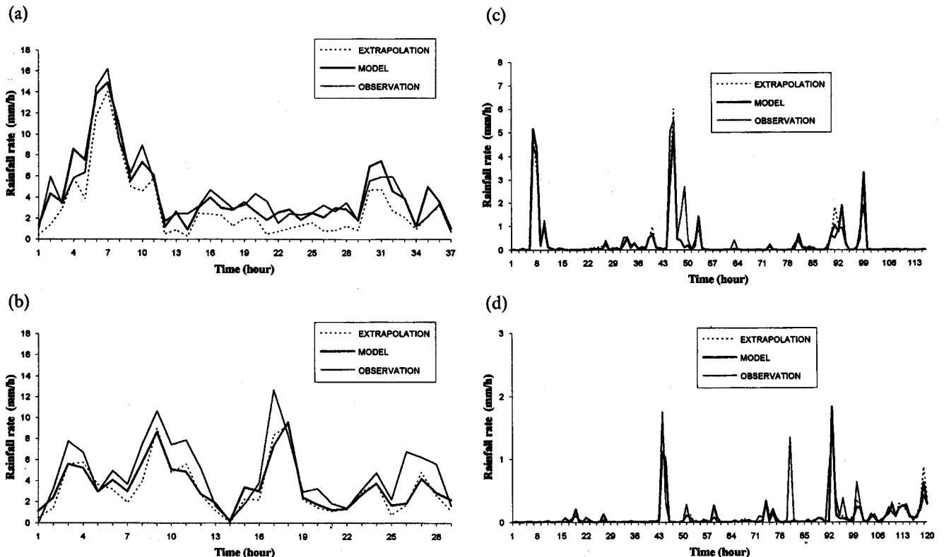
Fig. 3. Forecasted and observed rainfall rate for an one-hour lead-time a) NOV86 rain event b) OCT87 rain event c) OCT96 rain event d) NOV96 rain event.
