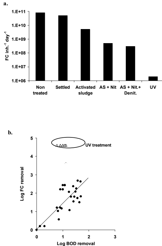
Fig. 2. (a) Specific loads of FC per inhabitant and per day for different types of wastewater treatment. AS = activated sludge process followed by decantation, AS + nit = activated sludge process with nitrification followed by decantation, AS + Nit + Denit = activated sludge process with nitrification and denitrification, UV = disinfection by UV irradiation added after secondary and tertiary treatment. (b) Removal of FC expressed in Log units plotted against removal of Biological Oxygen Demand in Log units for a number of investigated wastewater purification plants.
