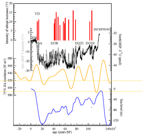
Fig. 2. NorthGRIP \delta^{18}\text{O} profile together with gas fractionation estimates of rapid temperature changes during rapid events. After Masson-Delmotte et al. (2005) with original data from NorthGRIP-community-members (2004); Huber et al. (2006); Landais et al. (2004); Severinghaus et al. (1998, 2003); Severinghaus and Brook (1999); Grachev and Severinghaus (2003). JJA 75°N insolation (orange line) is calculated after Berger and Loutre (1991). The global sea-level reconstruction (blue line) is from Waelbroeck et al. (2002).
