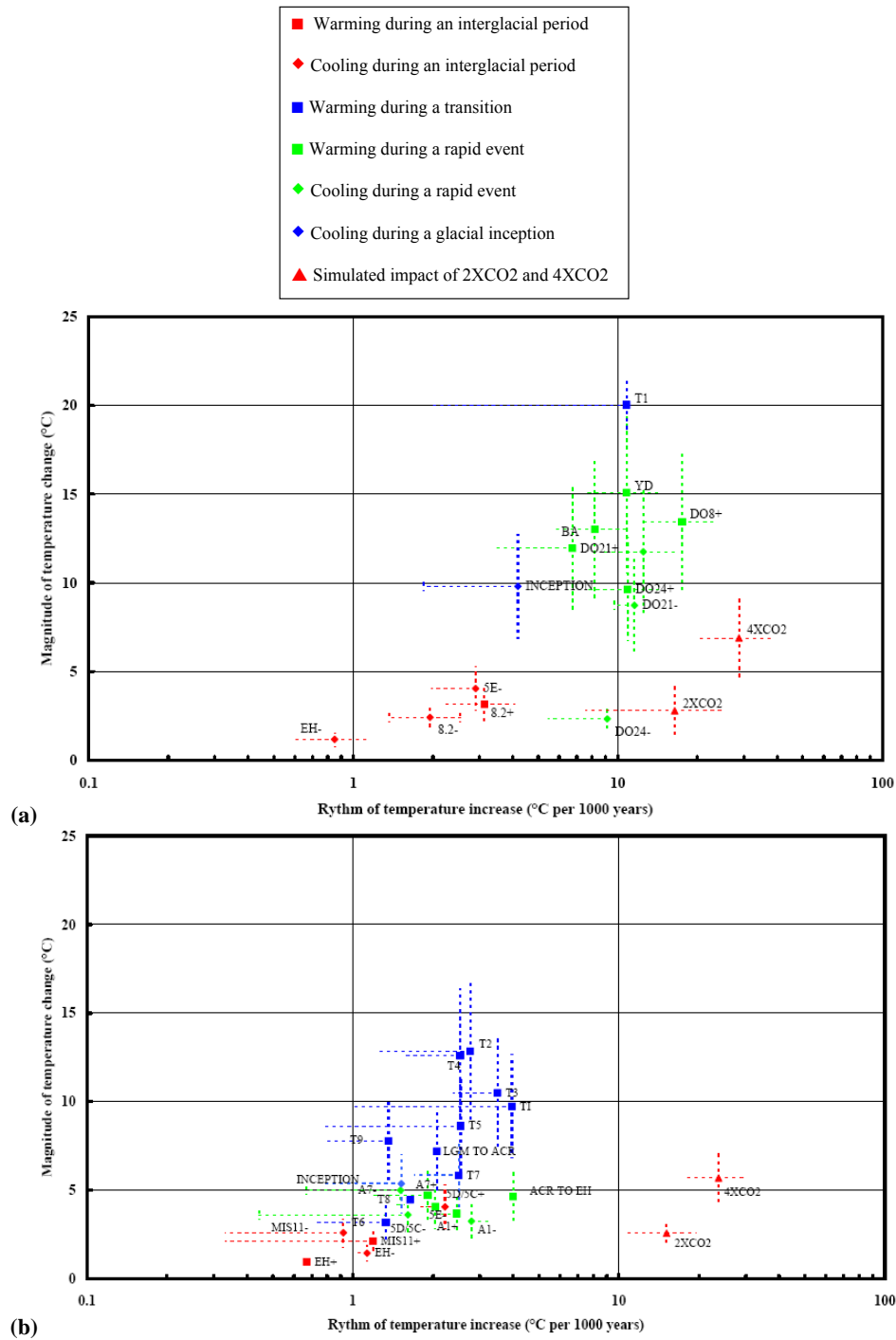
Fig. 7. Overview of the magnitude and rapidity of temperature changes in Greenland (a) and Antarctica (b) from ice core estimates and sensitivity studies conducted with coupled climate models (2×CO 2 and 4×CO 2 ). See text for details. EH(±) stands for warming/cooling before and after the Early Holocene temperature optimum (Masson-Delmotte et al., 2004); A1(±) for the warming/cooling before and after the A1 temperature maximum (Blunier and Brook, 2001); A7(±) for the warming/cooling before and after the A7 temperature maximum (Blunier and Brook, 2001); 5d/5c(±) for the warming/cooling before and after the first rapid event in Antarctica (Caillon et al., 2001); LGM for the Last Glacial Maximum; ACR for the Antarctic Cold Reversal; T1 to T9 for the terminations. These events are also located on the deuterium profile of EPICA Dome C on Fig. 3.
