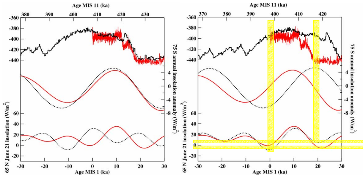
Fig. 6. Comparison of EPICA Dome C deuterium profile and orbital forcing for the past and future 30kyrs (red) and for a 60 kyr time period encompassing stage 11 (black). Two components of the orbital forcing are displayed: the anomalies from present-day of annual mean insolation at 75° S (basically corresponding to the obliquity signal) and the anomalies of mid-June insolation at 65° N. Different approaches have been developed to compare the transition from MIS 12 to MIS 11 and from MIS 2 to MIS 1. If the terminations are supposed to start simultaneously, this corresponds to a synchronisation of the obliquity fluctuations (left). This approach was followed by EPICA-community-members (2004). If the precession effect on 65° N mid-June insolation is synchronised, this places the terminations and the obliquity variations out of phase (right). This approach was initially suggested by Berger and Loutre (2002) and further followed by Ruddiman (2003). It has been suggested that thresholds on summer insolation are involved in the onset of ice ages. During the warm Antarctic episode corresponding to MIS 11, a first minimum of summer insolation is observed at ~420 ka. This minimum does not produce a glacial inception (horizontal dashed line labelled 1). The end of MIS 11 at Dome C corresponds to a second deeper minimum of summer insolation, at about 395 ka (horizontal dashed line labelled 2). It must be noted that the current minimum of mid-June insolation at 65° N lies between the first level (which did not cause the glacial inception in the beginning of MIS 11) and the second level (which corresponded to the end of MIS 11).
