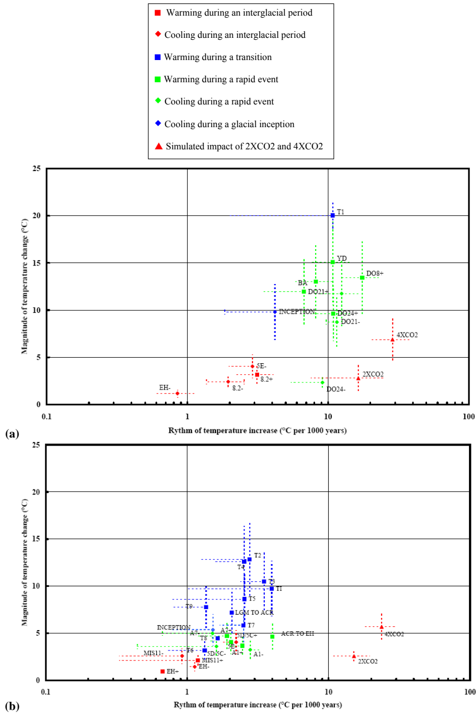
Fig. 7. Overview of the magnitude and rapidity of temperature changes in Greenland (a) and Antarctica (b) from ice core estimates and sensitivity studies conducted with coupled climate models ( 2\times\text{CO}_2 and 4\times\text{CO}_2 ). See text for details. EH( \pm ) stands for warming/cooling before and after the Early Holocene temperature optimum (Masson-Delmotte et al., 2004); A1( \pm ) for the warming/cooling before and after the A1 temperature maximum (Blunier and Brook, 2001); A7( \pm ) for the warming/cooling before and after the A7 temperature maximum (Blunier and Brook, 2001); 5d/5c( \pm ) for the warming/cooling before and after the first rapid event in Antarctica (Caillon et al., 2001); LGM for the Last Glacial Maximum; ACR for the Antarctic Cold Reversal; T1 to T9 for the terminations. These events are also located on the deuterium profile of EPICA Dome C on Fig. 3.
