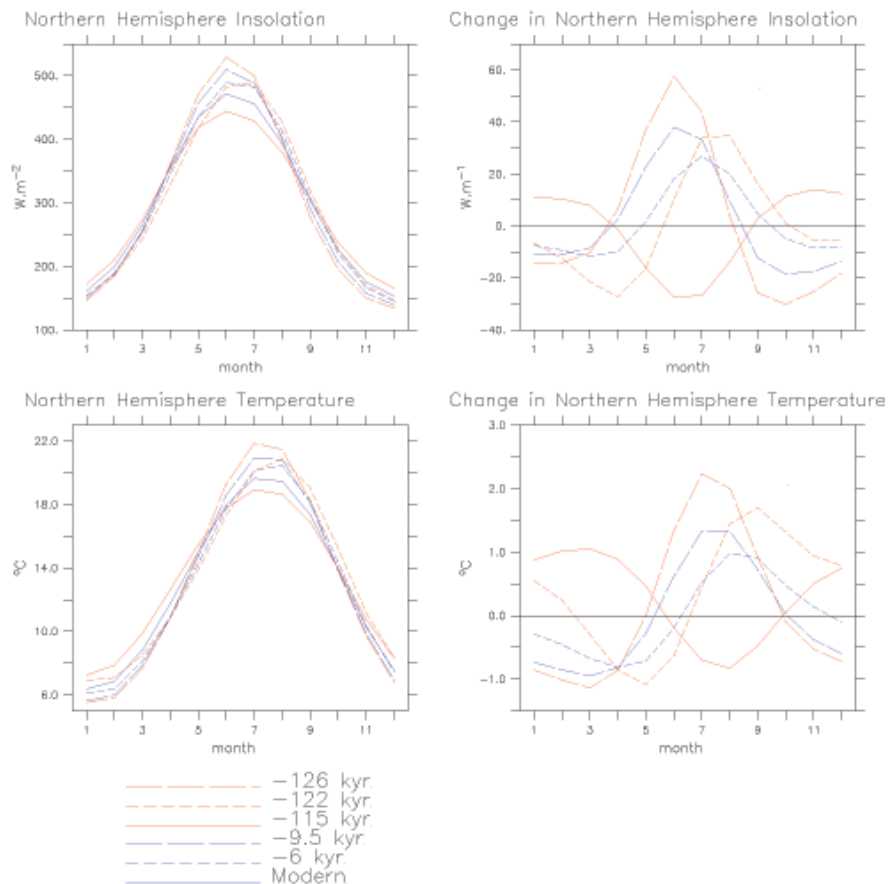
Fig. 2. (a) Insolation ( \text{W/m}^2 ) and (b) surface air temperature ( ^{\circ}\text{C} ) averaged over the Northern Hemisphere and plotted as a function of months. (b) and (c) Same as (a) and (b), both for the difference with the control simulation (0 ka).
