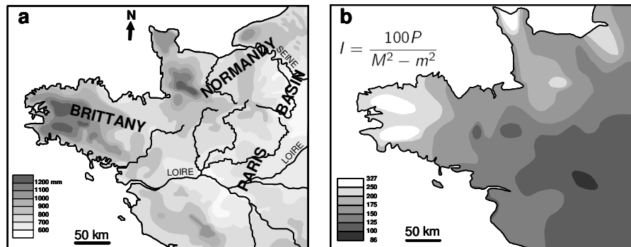
Fig. 1. (a) Average annual precipitation in north-western France for the climatological period 1961–1990, according to Kessler and Chambrud (1986) and MÉTÉO-FRANCE: Climate Normals 1961–1990, (b) Distribution of the Emberger index in northwestern France for the climatological period 1961–1990, according to Dubreuil (1994): P =Annual precipitation (mm), M =Average daily maximum temperature of the warmest month, m =Average daily minimum temperature of the coldest month.
