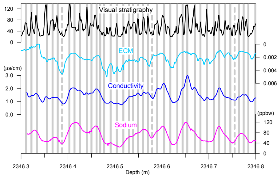
Fig. 2. Example of annual layer counting within the stadal preceding GI-14. Legend as for Fig. 1.
