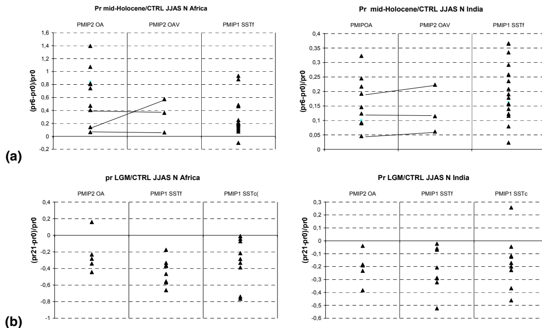
Fig. 8. Comparison of the JJAS change in precipitation simulated by PMIP2 and PMIP1 experiments respectively over Africa (20° W–30° E; 10° N–25° N) and North Indian (70° E–100° E; 20° N–40° N) for (a) mid-Holocene and (b) LGM. The lines link results of the same model when both OA and OAV simulations are available in the database.
