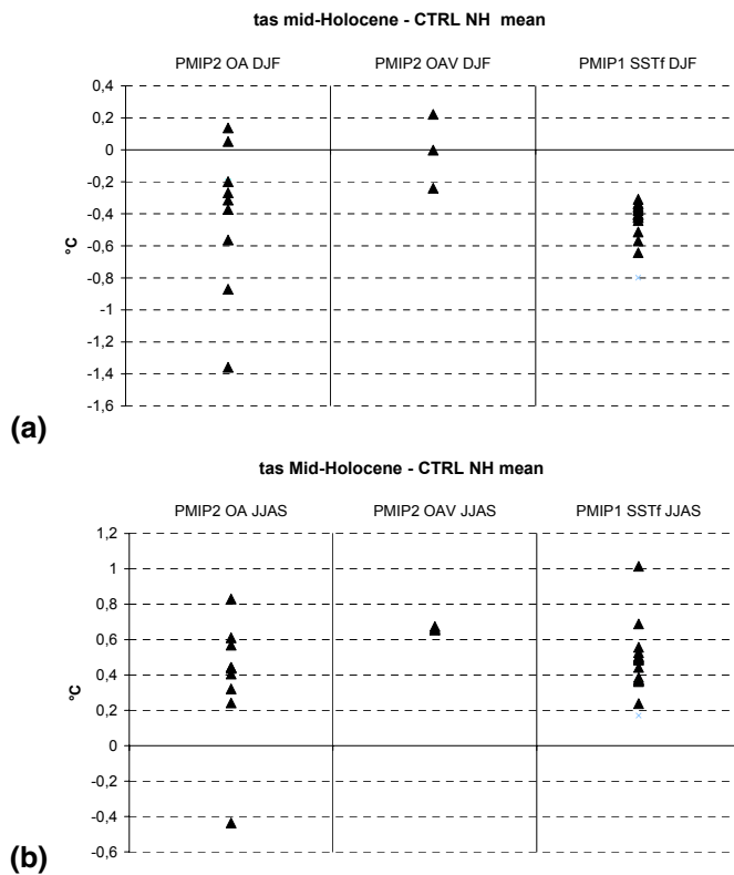
Fig. 4. As Fig. 2, but for DJF and JJAS mid-Holocene changes in air temperature averaged over NH.
