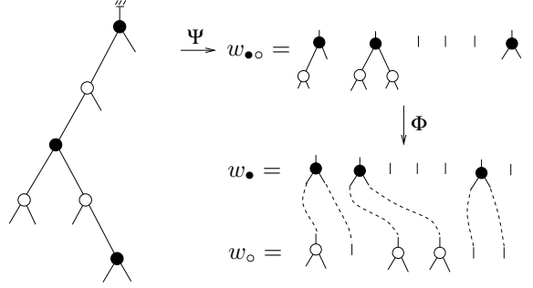
Fig. 9. A bicolor rooted binary tree, and the corresponding words w_{\bullet o} , w_{\bullet} , and w_o .
