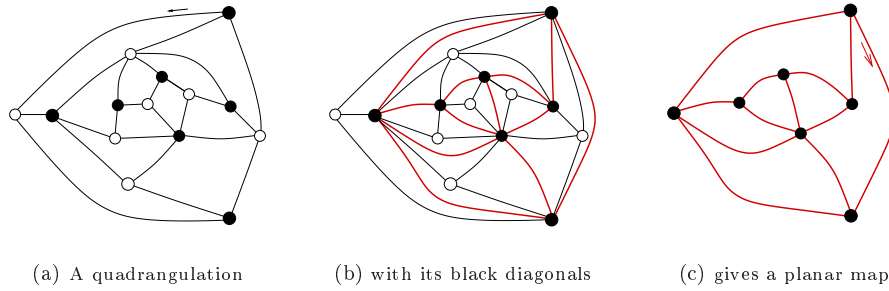
Fig. 2. The angular mapping: from a rooted irreducible quadrangulation to a rooted 3-connected planar map.
