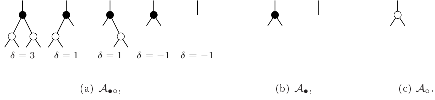
Fig. 8. The three alphabets for words associated to bicolored binary trees.
