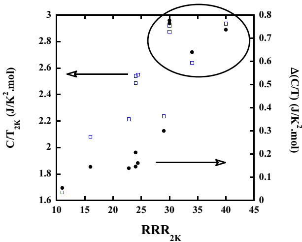
FIG. 4: C/T at 2 K and the total specific heat jump \Delta(C/T) defined in Fig. 1 versus RRR_{2K} . There is apparently a positive correlation between the three quantities. All the samples exhibiting clear double superconducting transitions (batches S1, L1 and L3) are within the large circle. They are of high quality : they are characterized by a large RRR_{2K} , a large C/T at 2 K and a large specific heat jump at the superconducting transition.
