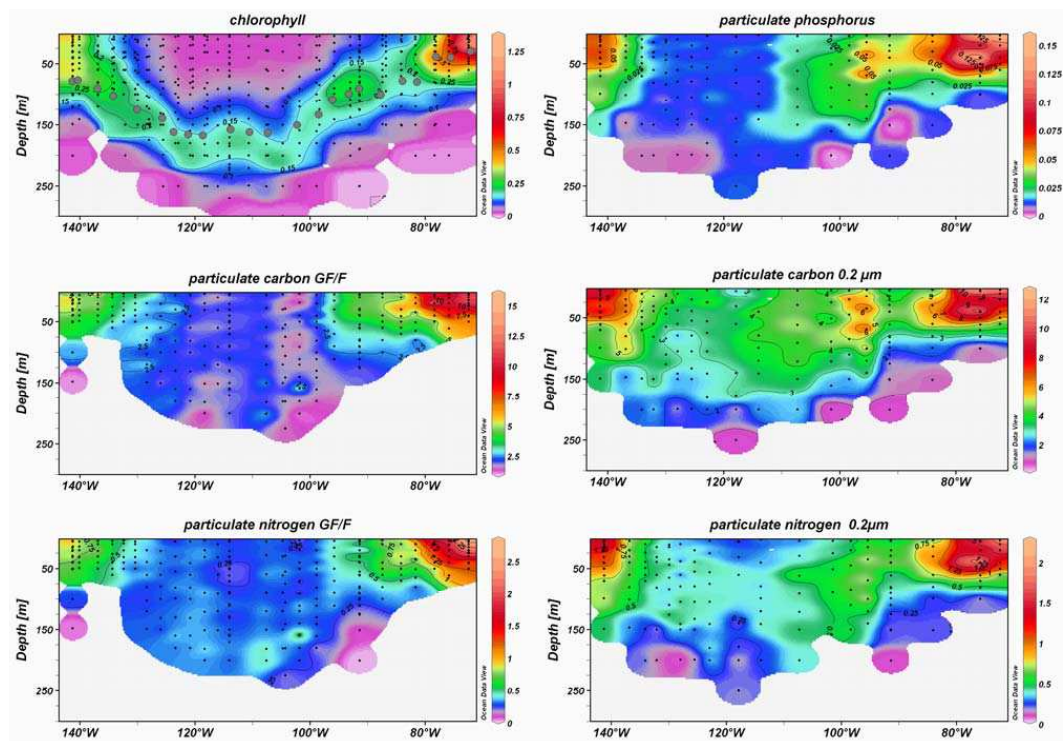
Fig. 3. Vertical sections of total chlorophyll- a (Chlorophyll in \mu\text{g l}^{-1} ), particulate phosphorus, >0.2 \mu\text{m} particulate organic carbon and particulate nitrogen and >\text{GF/F} particulate carbon and particulate nitrogen (units are in \mu\text{moles l}^{-1} ). Dark spots on chlorophyll section indicate the 1% light penetration depth. (Ocean Data View software (ODV), version 3.1, Reiner Schlitzer, http://odv.awi.de ).
