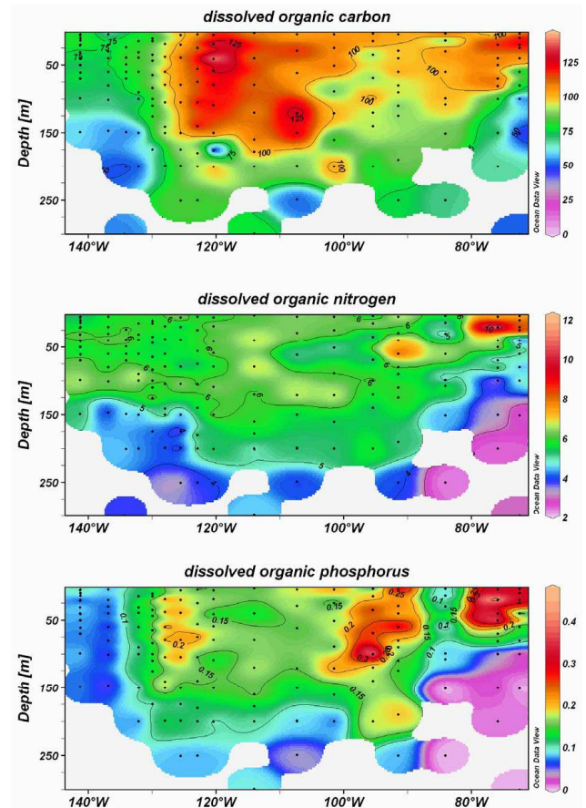
Fig. 9. Vertical section of dissolved organic carbon (DOC), dissolved organic nitrogen (DON) and dissolved organic phosphorus (DOP). Units are \mu\text{moles l}^{-1} (Ocean Data View software (ODV), version 3.1, Reiner Schlitzer, http://odv.awi.de ).
