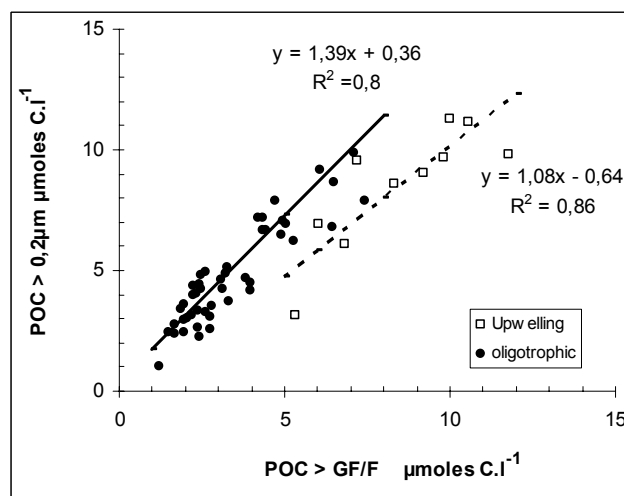
Fig. 5. Comparison between particulate organic carbon measured on 0.2 \mu\text{m} Teflon membranes by a wet-oxidation method (POC in \mu\text{moles}\ \text{l}^{-1} ) and particulate carbon on GF/F filters measured using High temperature combustion (PC in \mu\text{moles}\ \text{l}^{-1} ). Linear relationships are obtained using model II regression.
