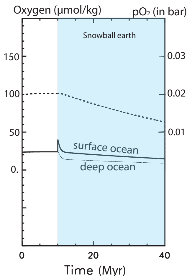
Fig. 3. Oxygen partial pressure during the glaciation with an ocean and atmosphere in steady state. The dash line represents the atmospheric O 2 mixing ratio, black lines being the surface and deep ocean oxygen concentrations. The blue bland represents the glaciation duration.
