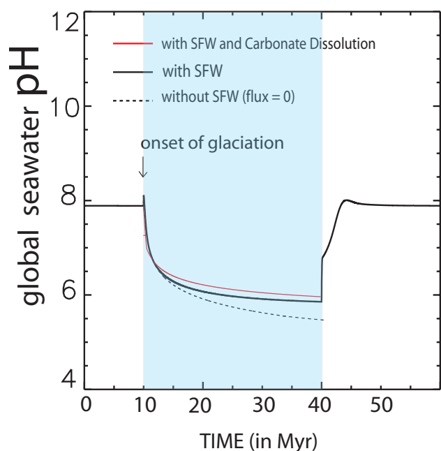
Fig. 5. pH evolution of the ocean during the glaciation. Snowball Earth begins after 10 Myr and lasts 30 Myr. All runs show, that during a snowball event, the seawater pH tends towards acidic values. Consequently, the seafloor weathering (SFW) increases its \text{CO}_2 consumption. By this way the pH is stabilized. The blue band represents the glaciation duration.
