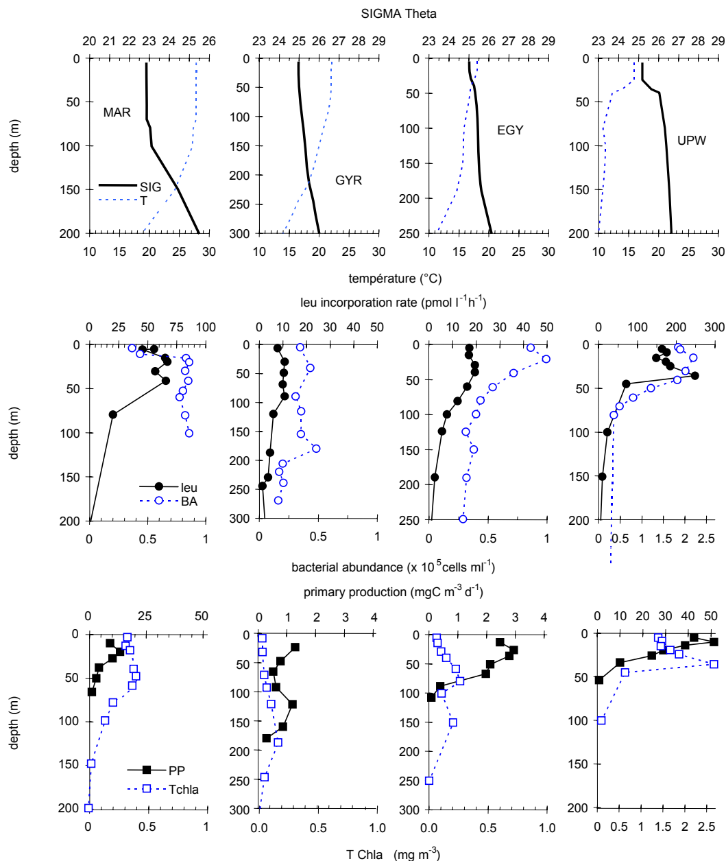
Fig. 3. Vertical distributions of temperature, sigma theta (upper panel), bacterial abundance, leucine incorporation rates (middle panel), Tchl a , primary production ( PP_{deck} , see methods, lower panel), at stations mesotrophic MAR (26 October), hyperoligotrophic GYR (12 November), oligotrophic EGYR (26 November), and eutrophic UPW (7 December). All variables are from the 09:00 CTD cast, except for bacterial abundance (the following 12:00 CTD cast).
