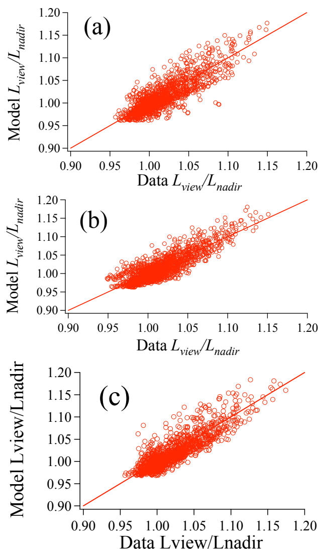
Fig. 7. Graph of model vs data of the ratio L_{\text{view}}/L_{\text{nadir}} for the BIOSOPE Station # 17; [Chl] was 0.11 \text{ mg m}^{-3} in the upper layer. (a) 412 nm, (b) 436 nm, and (c) 486 nm. The 1:1 line is also shown.
