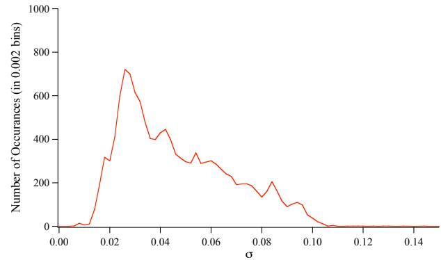
Fig. 6. Histogram of \sigma of the individual data points used in above comparison with the model.
