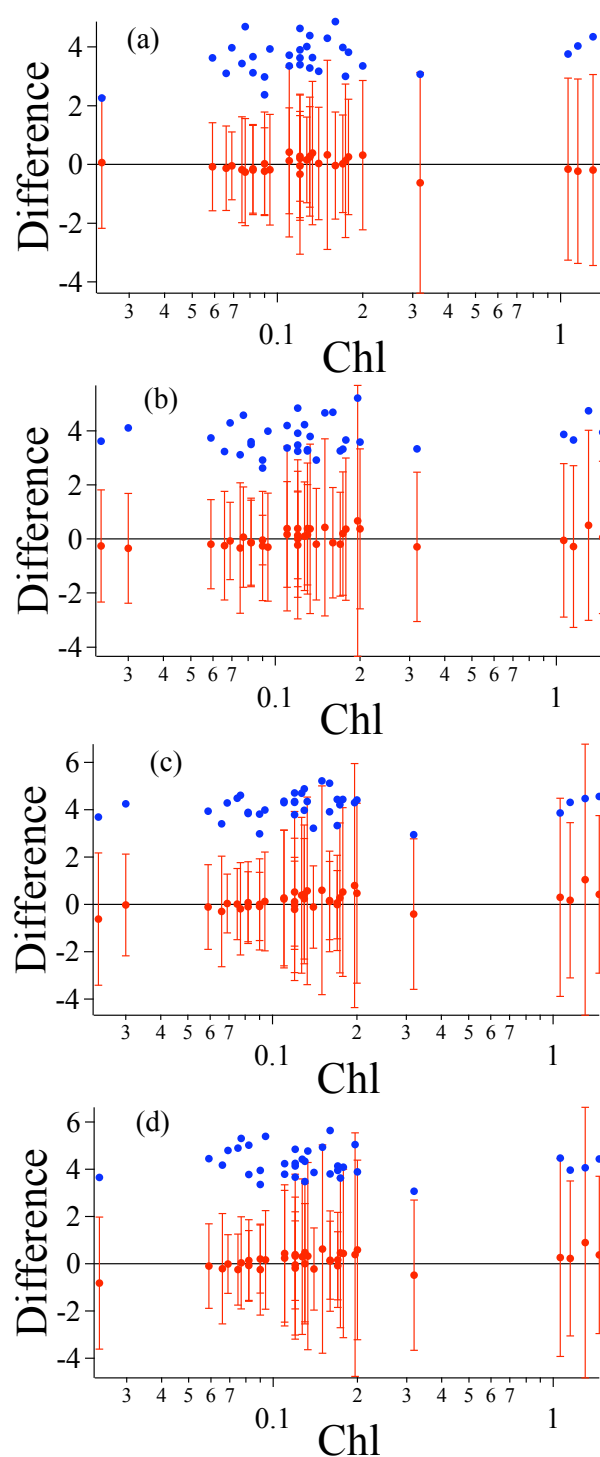
Fig. 8. Comparison for the entire data set between L_{\text{view}}/L_{\text{nadir}} the model and the data. (a) 412 nm, (b) 436 nm, (c) 486 nm, and (d) 526 nm. The red dots are the average difference in agreement between the model and the data. The bars on each data point are \pm 1 std. The blue dots are \sigma obtained in the image averaging process and represents the environmental noise in the images.
