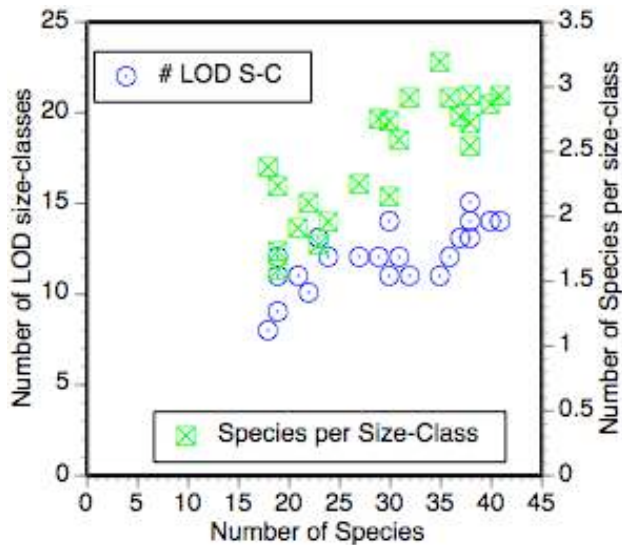
Fig. 6. Species packing in tintinnid communities across the SE Pacific Ocean. Comparing the different stations, both the number of mouth sizes, lorica oral diameter LOD in 4\text{ }\mu\text{m} size – class intervals, and the average number of species per mouth size increased with the number of species.
