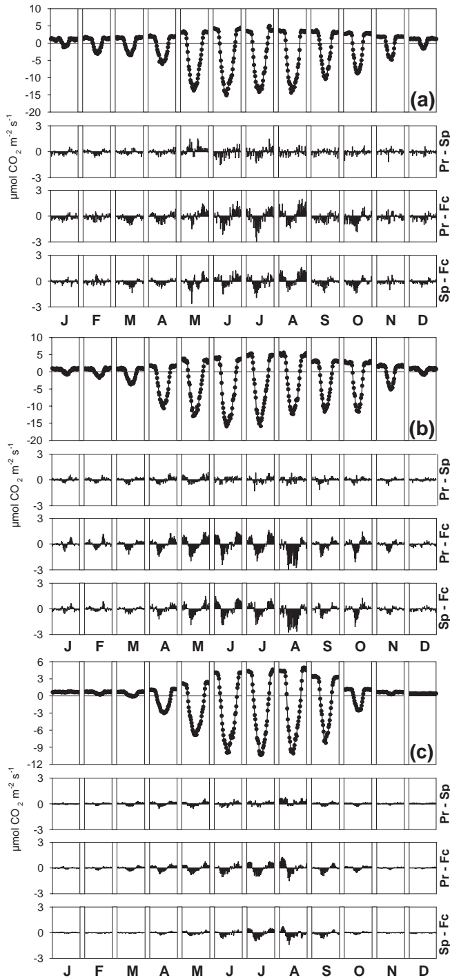
Fig. 5. Effect of different storage measurement methods on monthly mean diurnal NEE trends for three sites: BE01_01 (a), DE02_01 (b) and FI01_02 (c). In the upper panel diurnal cycle calculated from NEE_pr is shown; the other three panels the residuals respectively between the two storages (Pr-Sp), between storage from profile and no storage correction (Pr-Fc) and between storage from discrete approach and no storage correction (Sp-Fc).
