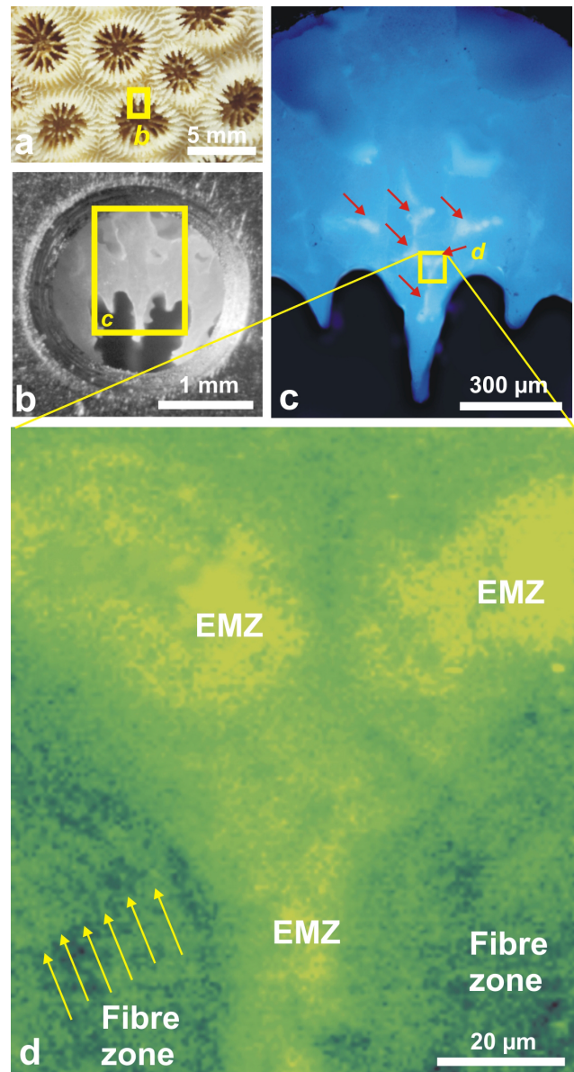
Fig. 7. Mapping of sulfated polysaccharides in Montastrea curta . (a) Morphology of the corallites. (b) Specimen in the sample holder. (c) Selection of the region to be mapped by UV fluorescence: the Early Mineralization zones show a strong response (red arrows). (d) Biochemical map of the selected zone. The Early Mineralization Zones exhibit a high sulfated polysaccharide concentration. In fibres, the well visible banding pattern in exact conformity with fibre growth layers (arrows) shows that mineral phase and sulfated polysaccharides are associated at a submicrometer scale within fibres.
