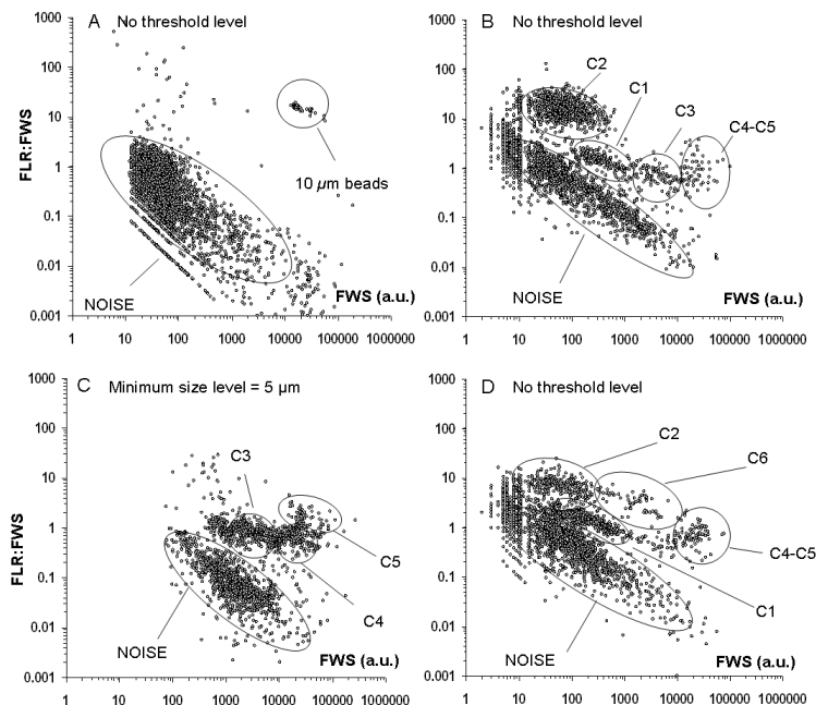
Fig. 4. Cytograms illustrating the cluster resolution. (a) FLR:FWS ratio (Red Fluorescence: Forward scatter) versus FWS for the analysis of 0.22\ \mu\text{m} filtered seawater supplemented with 10\ \mu\text{m} beads. No threshold level was applied so that the instrument noise could be recorded separately. (b) Same cytogram as in (a), related to the analysis of a pumped seawater sample. Four clusters were defined and labelled C1, C2, C3 and C4. (See Table 2 for the average values of their flow cytometric features). (c) Same cytogram as in (a) and (b) related to the analysis of a pumped seawater sample where a threshold was applied to the FWS signal in order to analyse a larger volume address larger cells like those in C3, C4 and C5. (d) Same cytogram as in (b), illustrating the resolution of C6.
