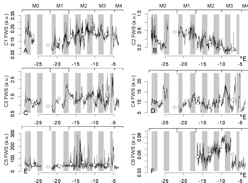
Fig. 7. Spatial variation along the ship track of the cell average forward scatter (FWS) for each cluster. White dots are the daily average value of the cell average FWS. Day and night periods are indicated with white and grey boxes respectively. The different water types crossed are specified on top of each plot.
