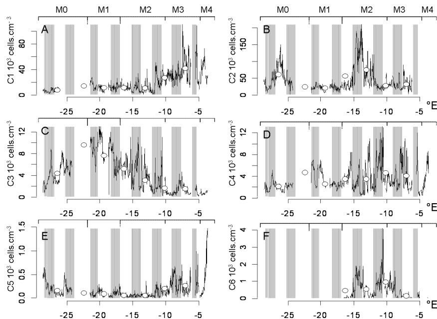
Fig. 5. Distribution of cell abundances for each resolved cluster along the ship track. White dots are the daily average value of abundances. Day and night periods are indicated with white and grey boxes respectively. The different water types are specified on top of each plot.
