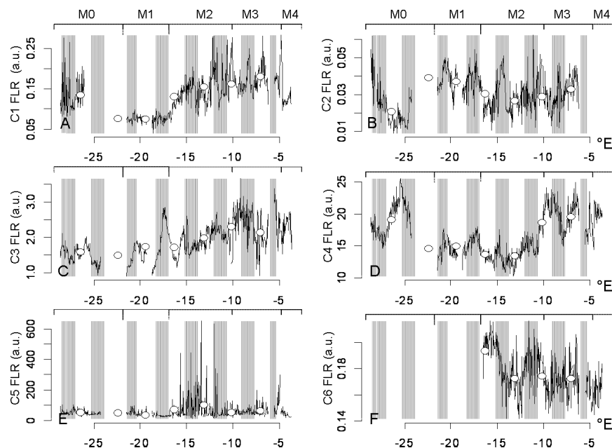
Fig. 6. Spatial variation along the ship track of the cell average red fluorescence (FLR) for each cluster. White dots are the daily average value of the cell average FLR. Day and night periods are indicated with white and grey boxes respectively. The different water types are specified on top of each plot.
