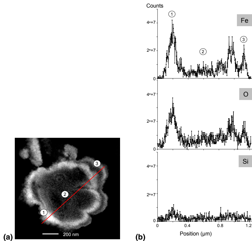
Fig. 8. (a) STEM pictures of the analysed particle exhibiting contrasted strata. The red line corresponds to the spectral profile line of 1.2 \mu\text{m} length. The numbers 1 to 3 indicate the points where the elemental quantitative analysis given in Table 5 was carried out. (b) Element specific spectra acquired along the red profile line. Points 1 to 3 are also indicated at their corresponding positions on the iron spectrum.
