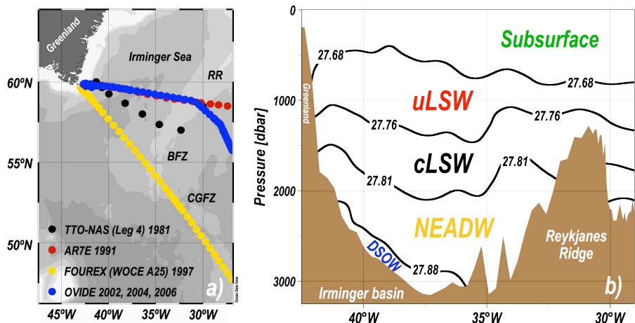
Fig. 1. (a) Map showing the Irminger Sea ends of the North Atlantic cruises used to assess the temporal evolution of the C_{\text{ant}} storage. The acronyms stand for: RR=Reykjanes Ridge, BFZ=Bight Fracture Zone and CGFZ=Charlie Gibbs Fracture Zone. (b) Main water masses (cLSW=classical Labrador Seawater; uLSW=upper Labrador Seawater; NEADW=North East Atlantic Deep Water; DSOW=Denmark Strait Overflow Water) present in the Irminger basin and analysed in terms of C_{\text{ant}} inventory distributions over time. The density ( \sigma_{\theta} in \text{kgm}^{-3} ) boundaries were established following Kieke et al. (2007) and Yashayaev et al. (2007).
