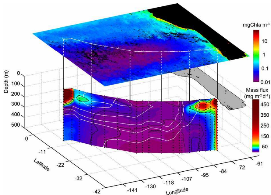
Fig. 5. Mass flux of LPM in \text{mg DW m}^{-2} \text{d}^{-1} estimated from size measurements of every individual particle recorded during the vertical deployment of the UVP. Only data from 0–500 m are shown for better visualisation of the superficial structures. The vertical resolution of the sampling was 10.5 L every 8 cm (see Guidi et al., 2007, for details). Isohalines are in white.
