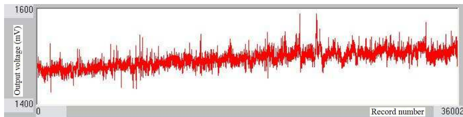
Fig. 1b. Example of high frequency record of CO 2 concentration (18 July 22:00 GMT) with intermittent turbulence.
