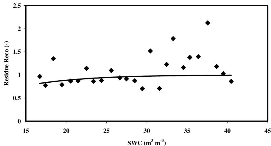
Fig. 4. Influence of the soil water content (first 10 cm depth) on the residues of the relationship between Reco and Ts_{10} . The dots correspond to the bin-averaged measurements for DSEFR and the line to the fit with a Gompertz function.
