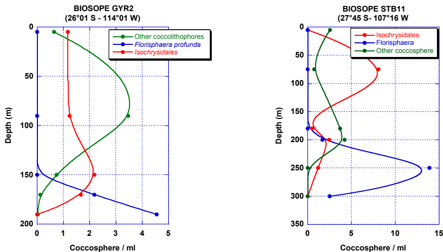
Fig. 10. Density in cells/ml of EGC (Isochrysidales) (red), Florispheera profunda (blue) and other coccolithophores (green) at station STB11 (right) and GYR2 (left).
