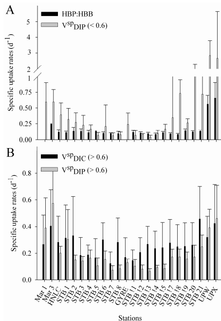
Fig. 5. (A) Bacterial specific uptake rates calculated from HBP:HBB ratio and V_{\text{DIP}}^{\text{SP}} in the fraction < 0.6 \mu\text{m} . (B) Phytoplankton specific uptake rates calculated from V_{\text{DIC}}^{\text{SP}} and V_{\text{DIP}}^{\text{SP}} in the fraction > 0.6 \mu\text{m} . Average specific uptake rates values on the photic zone. Autotrophic biomass calculated from Chla using C:Chla conversion factors as describe in the Materials and Methods section. Heterotrophic bacterial biomass calculated from bacterial cells abundance converted to C equivalent using a conversion factor of 10 \text{ fgC cell}^{-1} .
