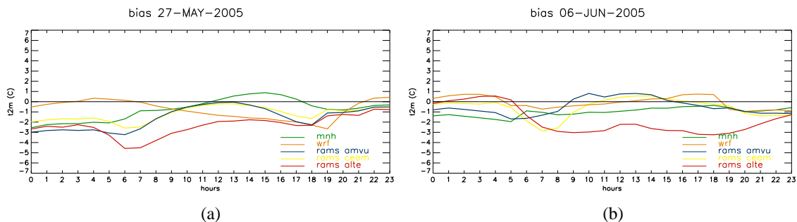
Fig. 2. Temporal evolution of the bias calculated for each model for the temperature at 2m (T2M) on (a) 27 May and (b) 6 June.
