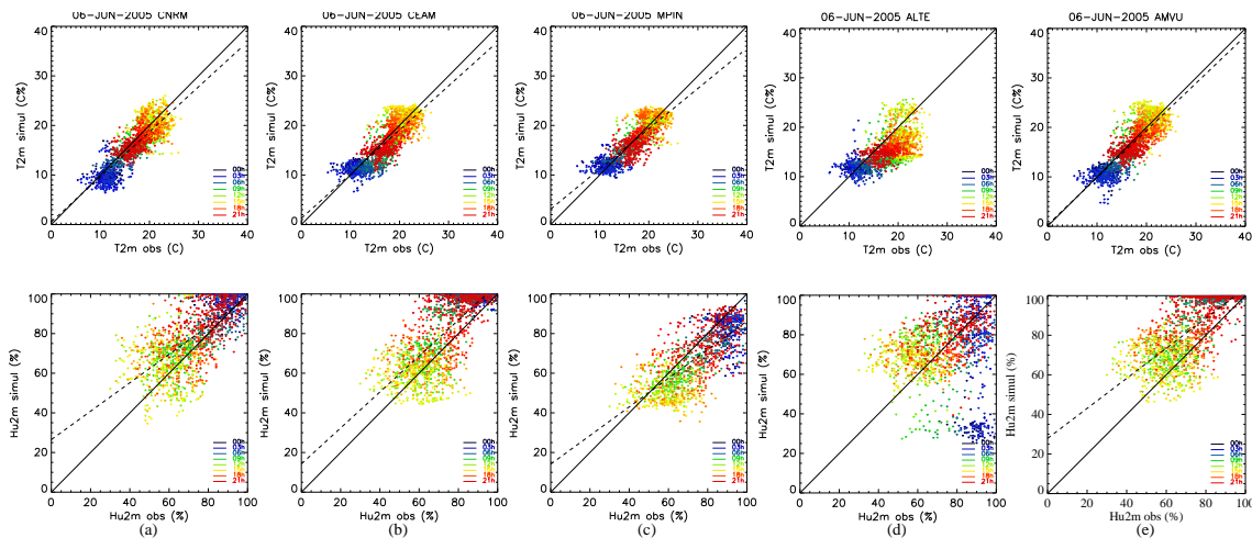
Fig. 4. Temperature at 2 m and relative humidity at 2 m simulated vs observed for each model. Each point represents one hour for one station, i.e. 82 stations \times 24 h on 6 June. (a) MNM-CNRM, (b) RAMS-CEAM, (c) WRF-MPI, (d) RAMS-ALTE, (e) RAMS-AMVU.
