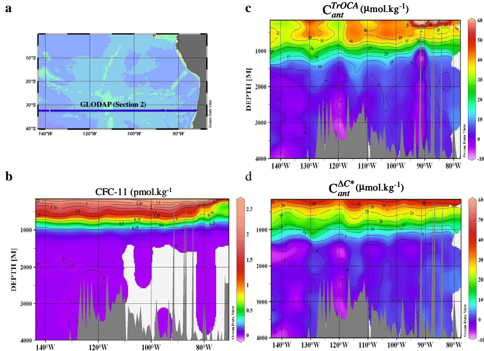
Fig. 6. Vertical distribution on the Sect. 2 of the GLODAP data of the anthropogenic CO 2 estimated with the TrOCA approach ( C_{ant}^{TrOCA} and the \Delta C^* approach ( C_{ant}^{\Delta C^*} ) and the anthropogenic tracer the CFC-11: (a) Location of the Sect. 2 of the GLODAP data, (b) CFC-11, (c) C_{ant}^{TrOCA} , (d) C_{ant}^{\Delta C^*} .
