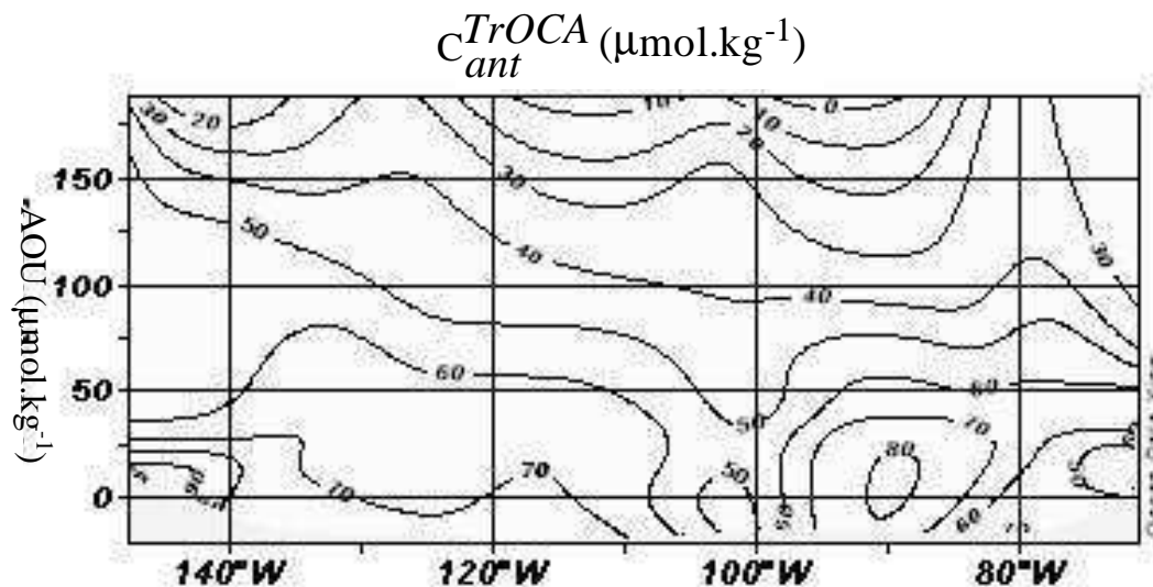
Fig. 4. Section of C_{ant}^{TrOCA} interpolated onto a vertical co-ordinate of AOU.
