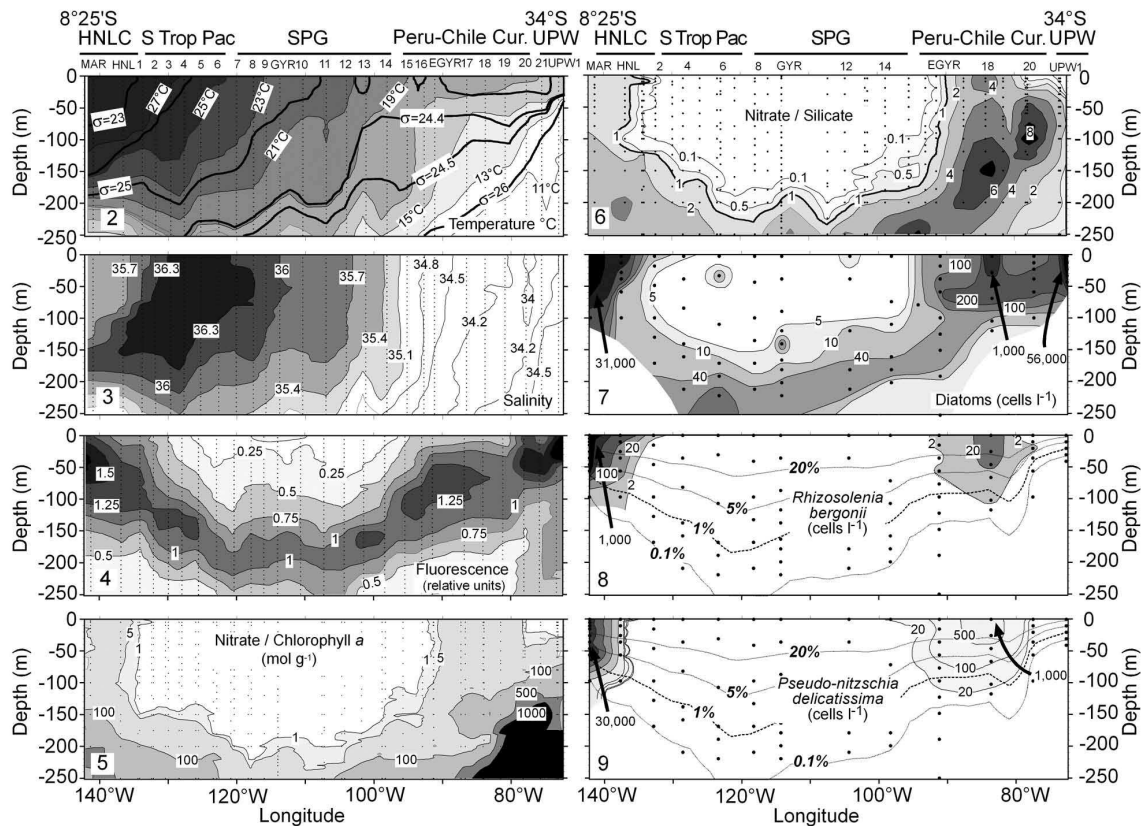
Figs. 2–9. Section plots of (2) temperature ( ^{\circ}\text{C} ) and the isopycnals lines labelled in units of sigma-t (density-1000)( \text{kg m}^{-3} ) are shown. (3) salinity. (4) fluorescence (relative units). (5) Nitrate-chlorophyll a ratio (6) Nitrate-silicate ratio; (7) abundance ( \text{cells l}^{-1} ) of diatoms. (8) Rhizosolenia bergonii and (9) Pseudo-nitzschia delicatissima . The dashed lines represent the percentage of the surface irradiance.
